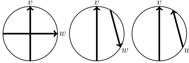
FIGURE 2. When \beta(v, w) = 0 .
