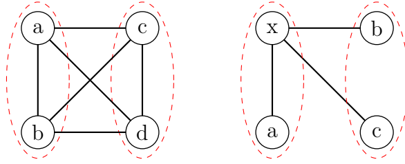
FIGURE 3. Splits in K_4 and the Claw
