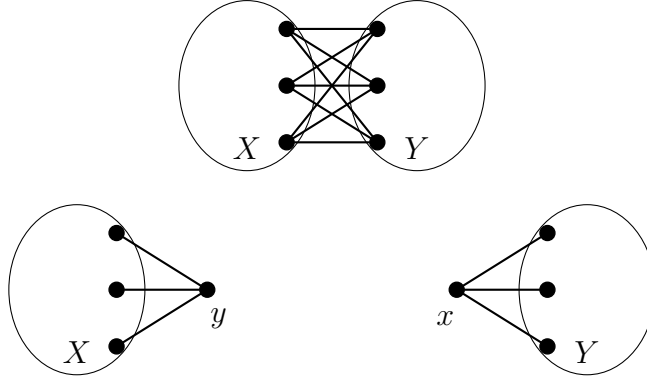
FIGURE 4. G , G_1 , and G_2
