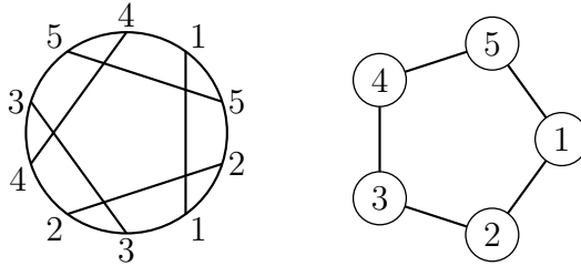
FIGURE 1. A Chord Diagram and its Circle Graph
