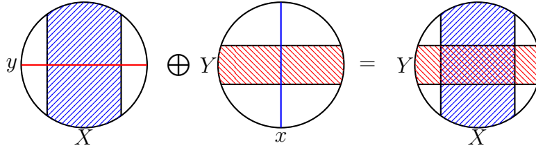
FIGURE 5. Chord diagrams for G_1 , G_2 and G
